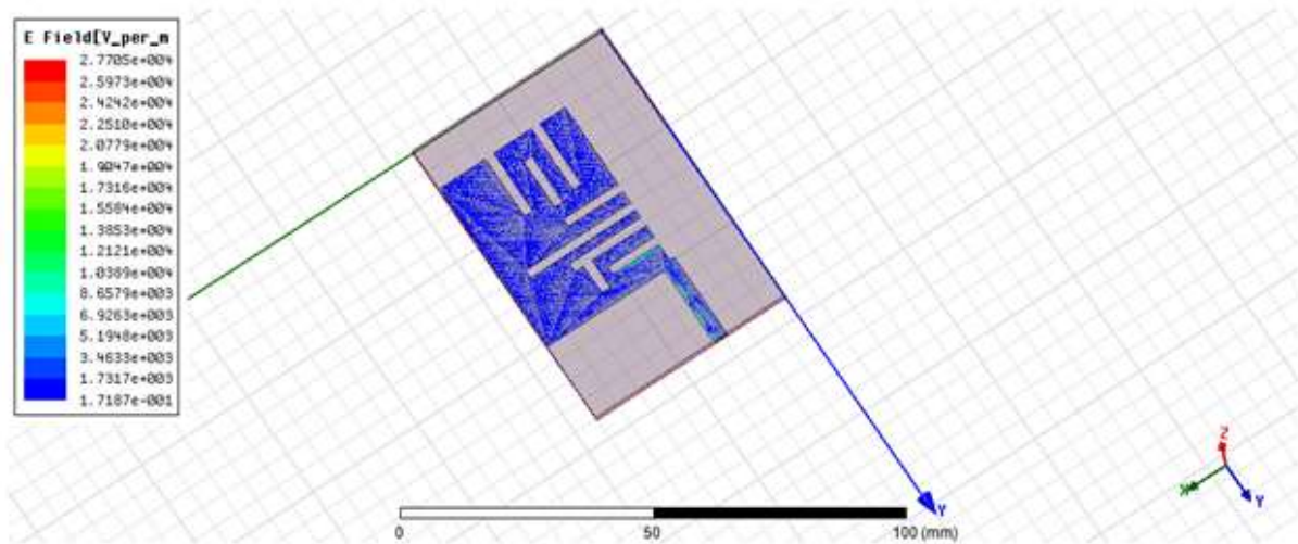
Fig 5 E-field Distribution
