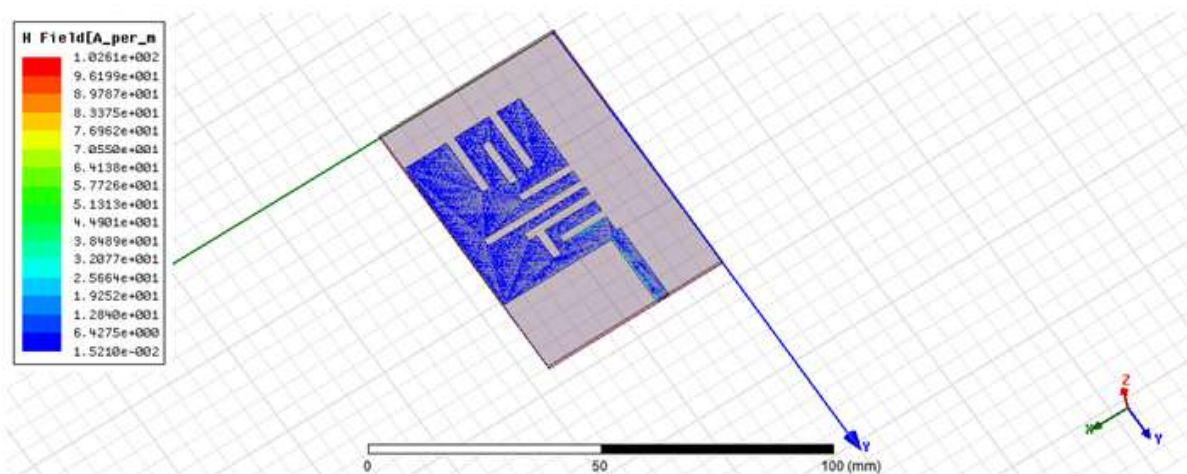
Fig 6 E-field Distribution
