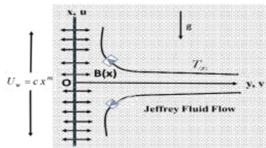
Figure 1. Physical model
